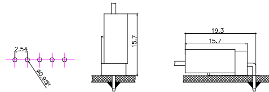
安装尺寸 MOUNTING MEASUREMENT
